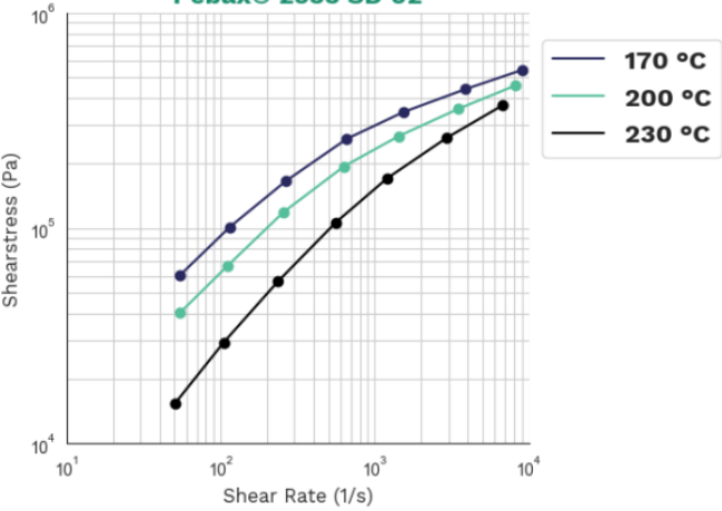
Shearstress-shear rate Pebax® 2533 SD 02
