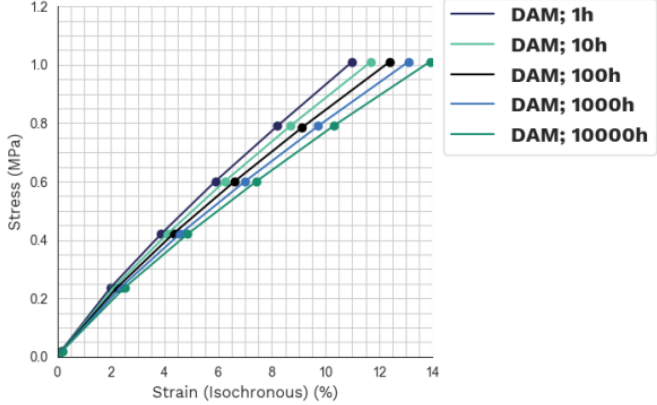
Stress-strain (Isochronous) 23 °C Pebax® 2533 SD 02
