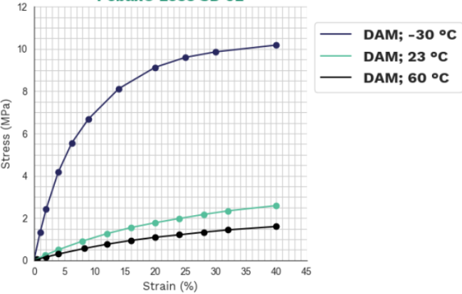
Stress-strain Pebax® 2533 SD 02
