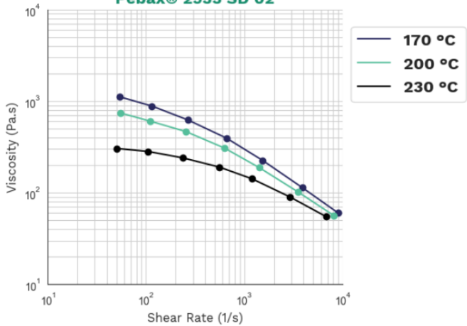
Viscosity-shear rate Pebax® 2533 SD 02
